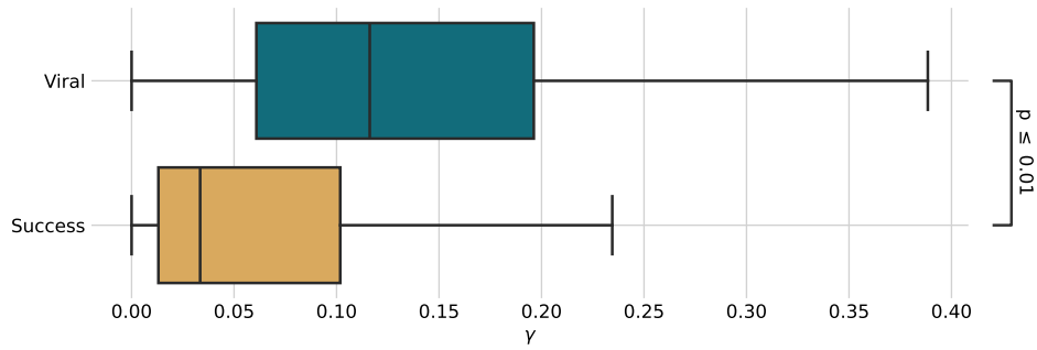
Figure 5. \gamma values for virality and success curves using the SIR model. Significance is calculated using the Mann-Whitney U test (p-value = 1.435\text{e-}104 ). Outliers are omitted for visual clarity (viral has 65 outliers, maximum is 1.780; success has 231 outliers, maximum is 5.359).
