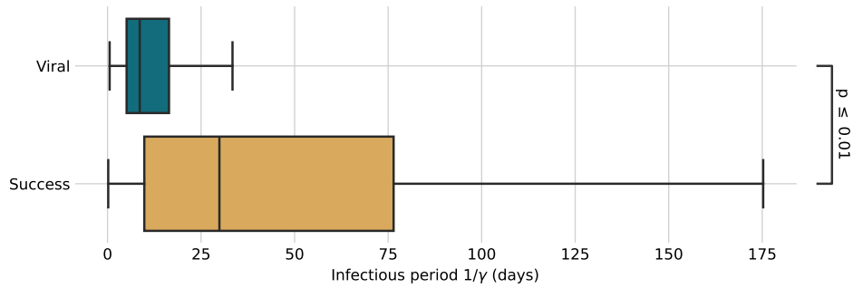
Figure 6. Infectious period for virality and success curves using the SIR model. Significance is calculated using the Mann-Whitney U test (p-value = 1.435\text{e-}104 ). Outliers are omitted for visual clarity (viral has 104 outliers, maximum is 1.313\text{e+}20 ; success has 57 outliers, maximum is 3.047\text{e+}17 ).
