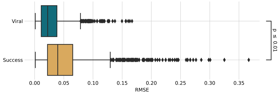
Figure 3. RMSE for virality and success curves using the SIR model. Significance is calculated using the Mann-Whitney U test ( p\text{-value} = 1.845e\text{-}64 ).
