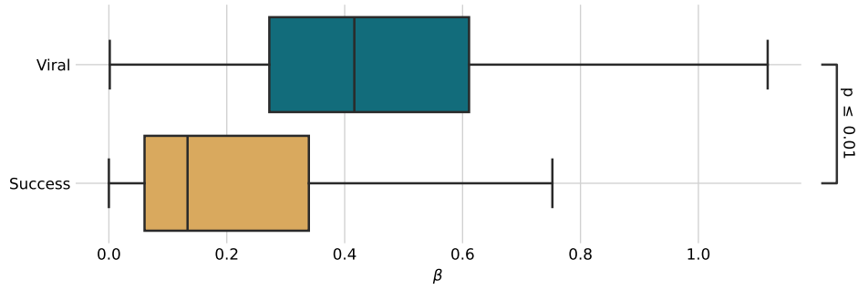
Figure 4. \beta values for virality and success curves using the SIR model. Significance is calculated using the Mann-Whitney U test (p-value = 3.875e-139). Outliers are omitted for visual clarity (viral has 137 outliers, maximum is 3.155; success has 118 outliers, maximum is 10.716).
