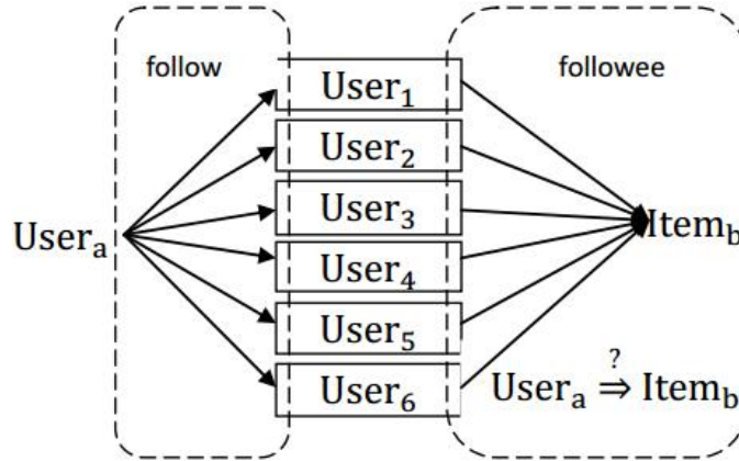
Figure 1. Relationship f_{out}(A) \cap f_{in}(B)
