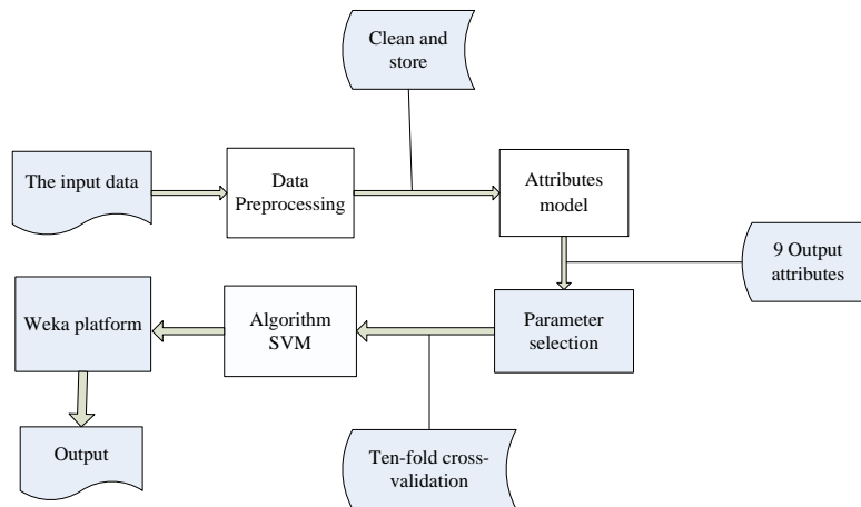
Figure 3. The flow-process diagram of recommender system
