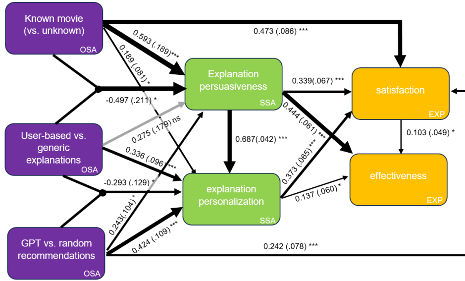
Figure 2. Path model showing how persuasiveness and personalization are influenced by objective system aspects (OSA) and how they predict satisfaction and effectiveness. Line thickness represents coefficient strength. Standard errors in brackets. Significance: * p < .05 , ** p < .01 , *** p < .001 .
