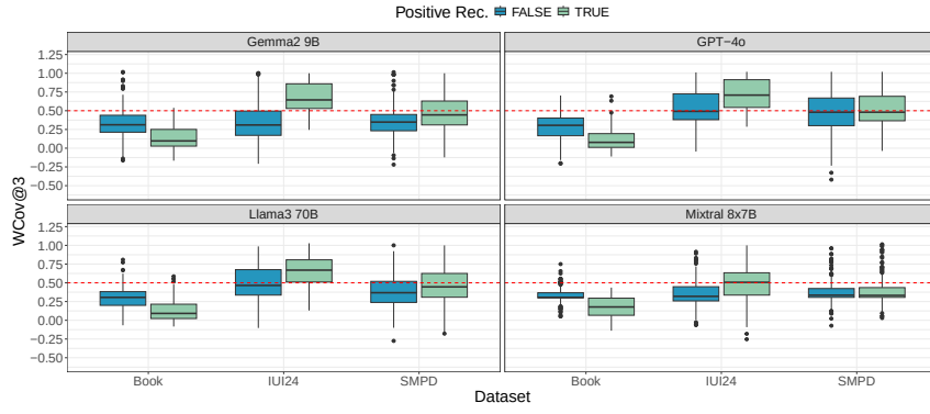
Figure 3. Distribution of the Weighted Coverage at Top-3 for the four models and three datasets.
