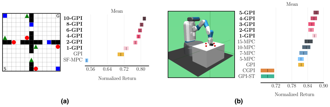
Figure 4. Mean normalized performance over test tasks in the (a) FourRoom and (b) robotic arm (FetchPush) domain. The performance of h -GPI increases significantly as the planning horizon ( h ) increases.
