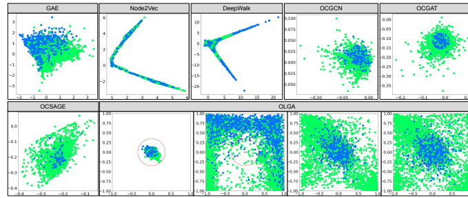
Figure 1. OLGA interpretable results.
