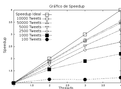
Figura 3. Speedup
