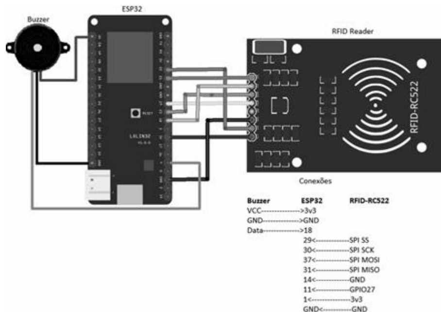
Figura 4 — Layout ESP32, RFID Reader e buzzer.
