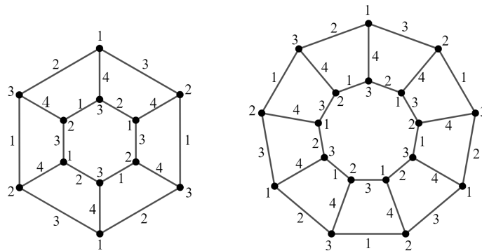
Figure 2. Circular ladder graphs L_{12} and L_{18} with non-equitable 4-total colorings.
