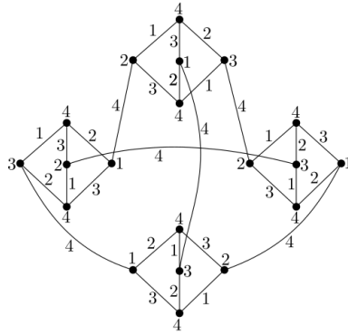
Figure 1. A non-equitable 4-total coloring of graph R .
