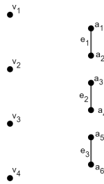
Figure 4. Diagram of case with 4 vertices and 3 edges in a total independent set of 7 elements, considering a graph with n = 10 vertices.
