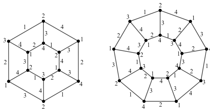
Figure 3. Circular ladder graphs L_{12} and L_{18} with equitable 4-total colorings.
