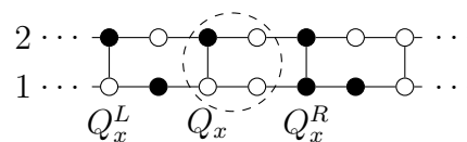
(b) An example where Rule (R2) is applied.
