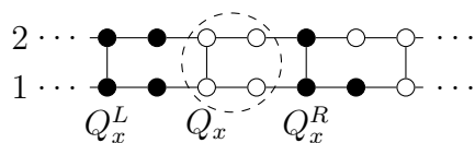
(a) An example where Rule (R1) is applied.
