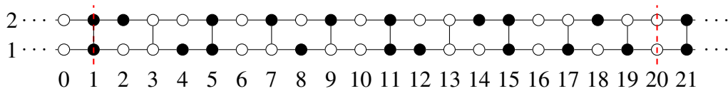
Figure 1. Pattern of an identifying code for H_2 , whose density is 9/20 .
