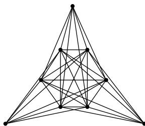
Figure 1. A graph with treewidth 6 and average degree 22/3 .
