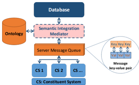
Fig. 4. Ontology-based Integration Architecture
