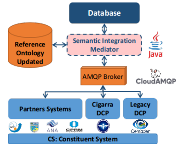
Fig. 5. High-level implementation of the Ontology-based Integration
