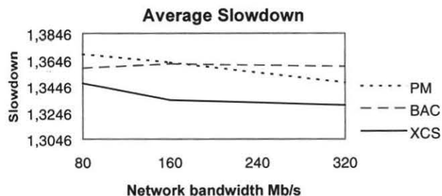
Figure 4 – Average Slowdown of the policies for the values of network bandwidth
