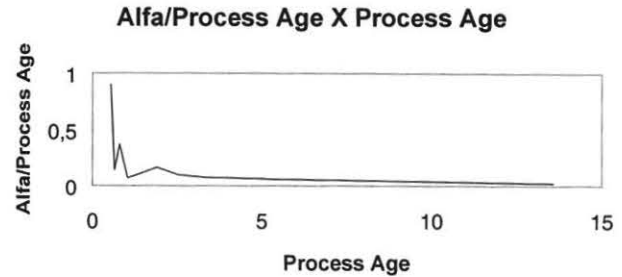
Figure 8 – Ratio Alfa / Process Age given by Methusela+XCS for processes greater than 0.5 second
