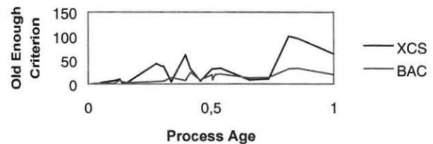
Figure 9 – How Methusela+XCS and Analytic Criterion decide if a process is old enough for migration.
