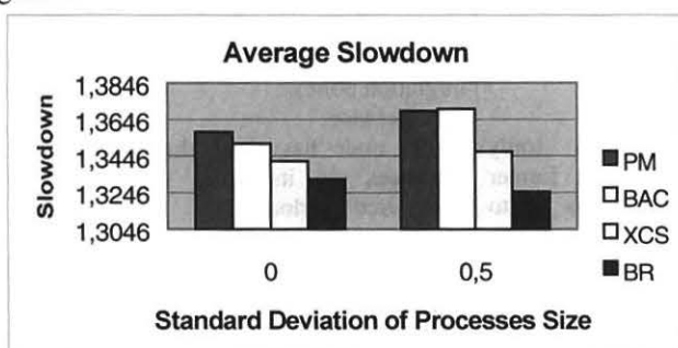
Figure 3 – Average Slowdown of the policies for the values of standard deviation of processes size
