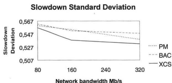
Figure 5 – Slowdown Standard deviation of the policies for the values of network bandwidth
