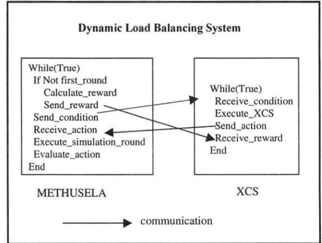
Figure 2 – Interaction between Methusela and XCS
