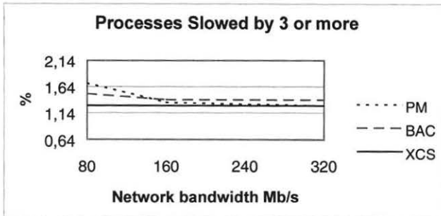
Figure 6 – Processes Slowed by 3 or more of the policies for the values of network bandwidth
