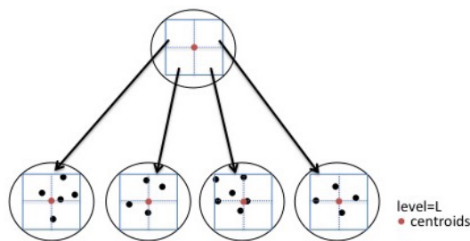
Figure 2. Quadtree node representation
