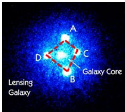
Figure 1. Einstein Cross identification from astronomic catalogs
