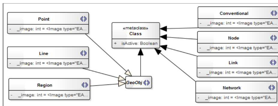
Figure 2. UML GeoOOA profile
