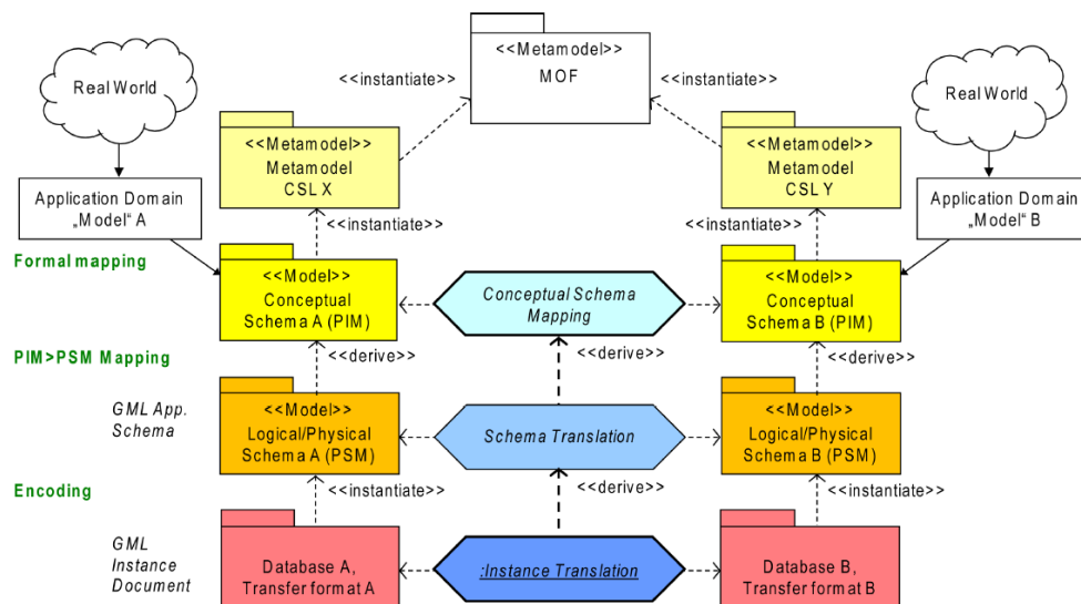
Figure 1. Schema interoperability [Staub 2007]
