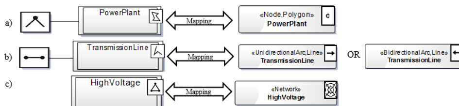
Figure 4. Mapping between MDG_GeoOOA and MDG_GeoProfile
