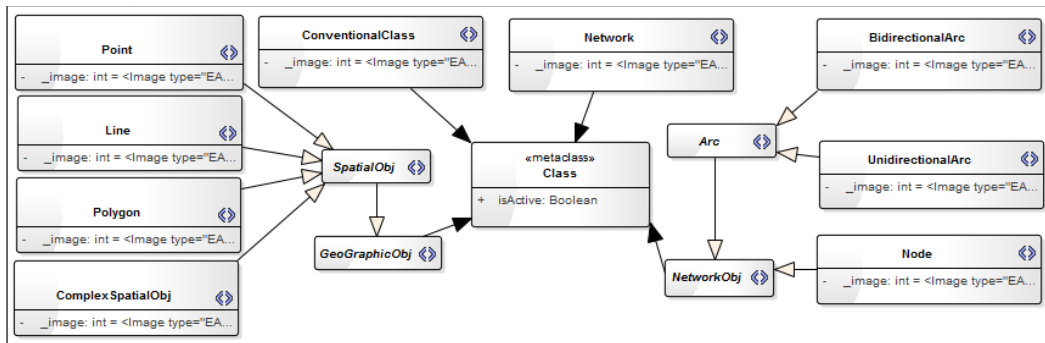
Figure 3. UML-GeoFrame profile
