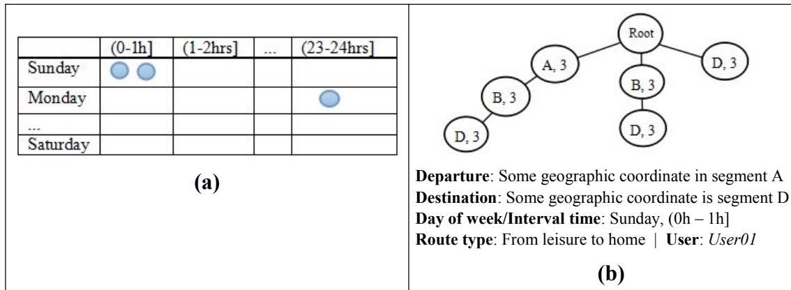
Figure 1: (a) Trajectory models matrix; (b) Content of a trajectory model
