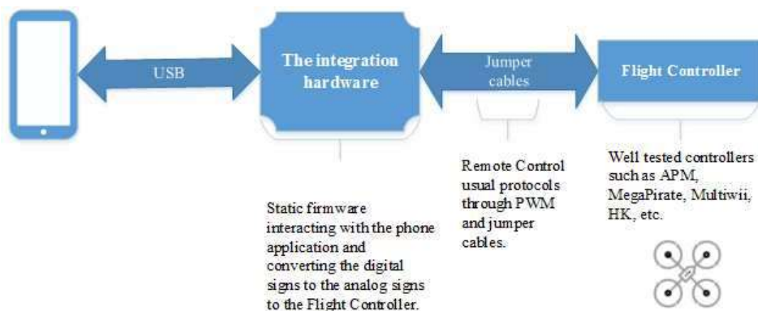
Figure 1: The hardware architecture of the UAV.
