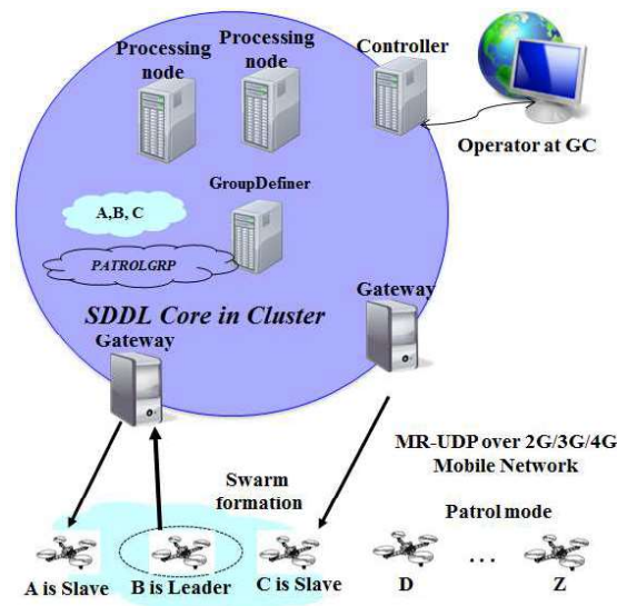
Figure 2: Components of the SDDL middleware involved in the UAV communication and group management.
