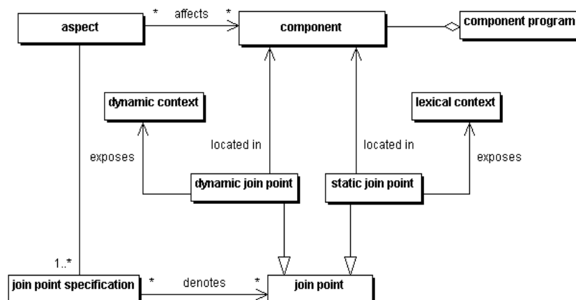
Figure 3: The join point model
