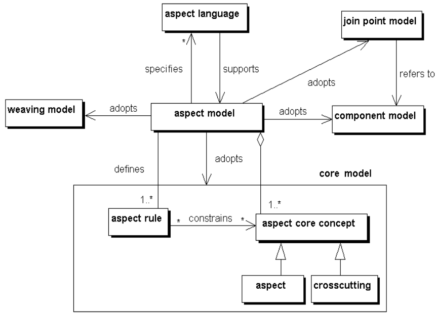
Figure 1: The aspect model
