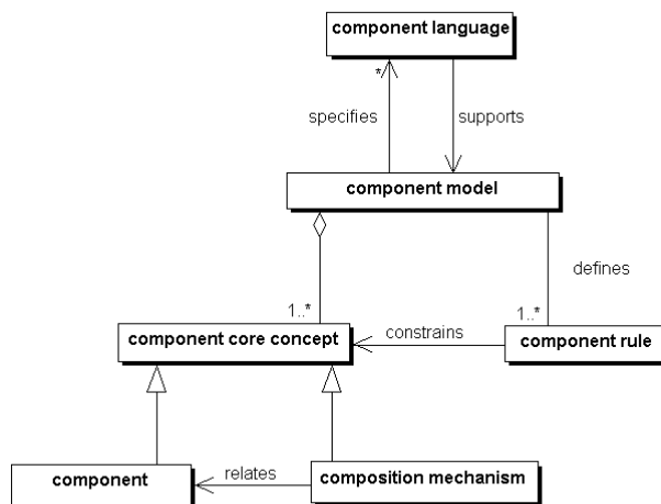
Figure 2: The component model
