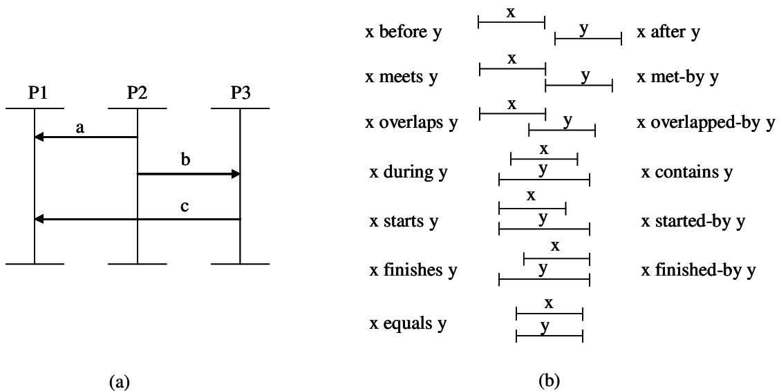
Figure 1: A Basic MSC and Allen's Basic Interval Relations
