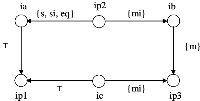
Figure 4: The resulting ICN
