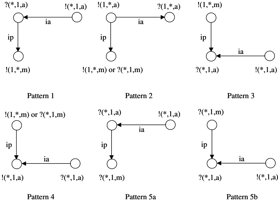
Figure 3: Basic patterns of a labeled MSC
