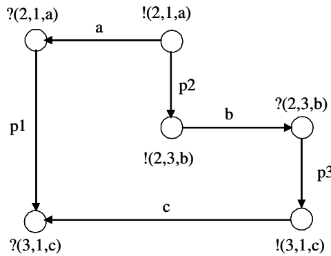
Figure 2: The partial order of the MSC of Figure 1
