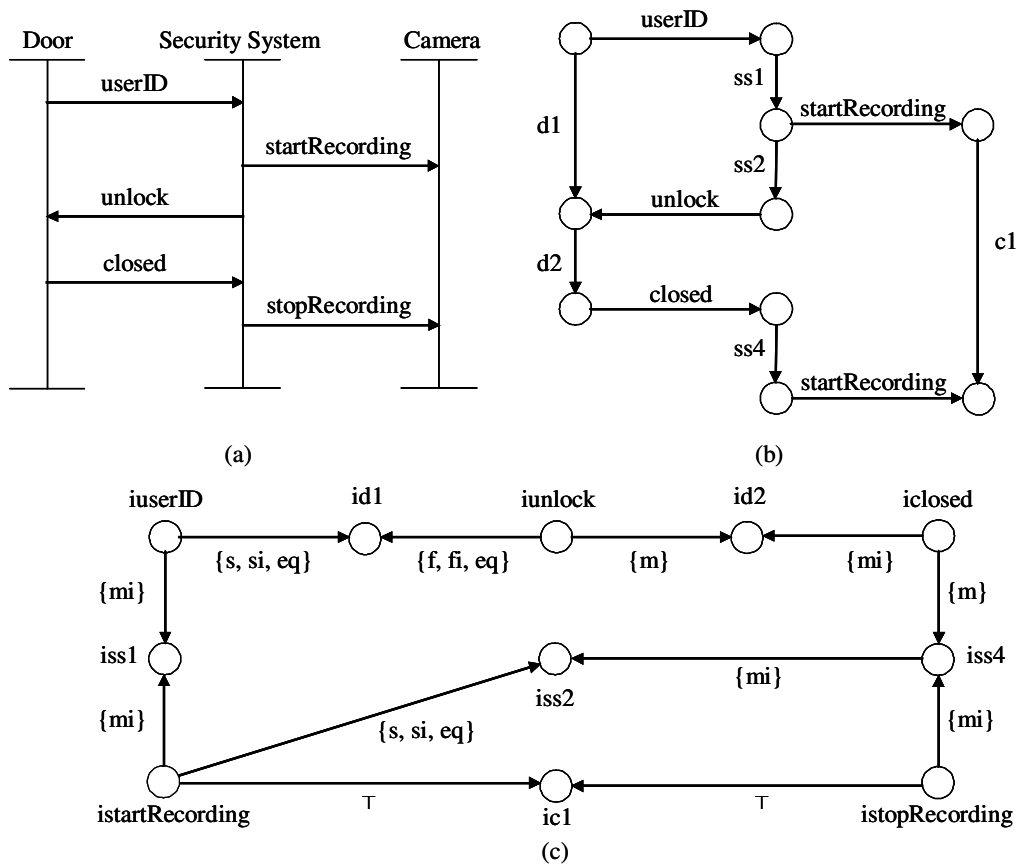
Figure 5: A simple secure building control MSC, its visual order and ICN
