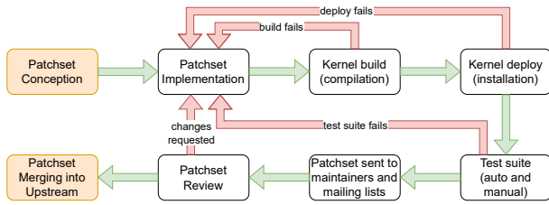
Figure 6: Concept map of the patchset development workflow.
