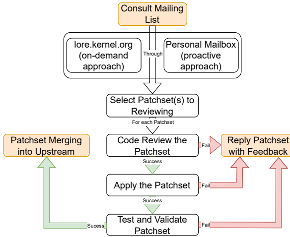
Figure 7: Concept map of the patchset reviewing workflow.
