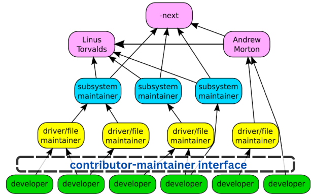
Figure 1: Patches flow into the mainline [9].
