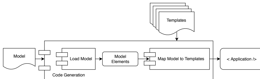
Figure 4. Model-to-code transformation.
