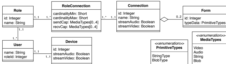
Figure 3. Metamodel for runtime models.
