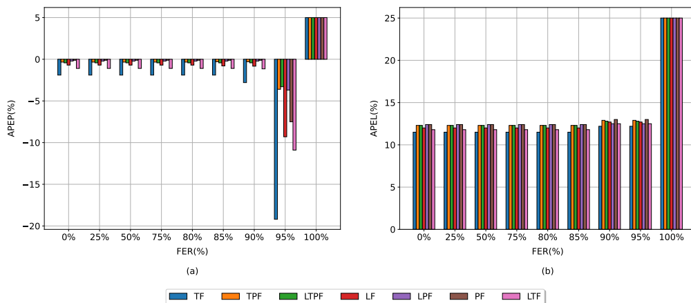
Figure 4. APEP metric for a Medium Speed scenario.
