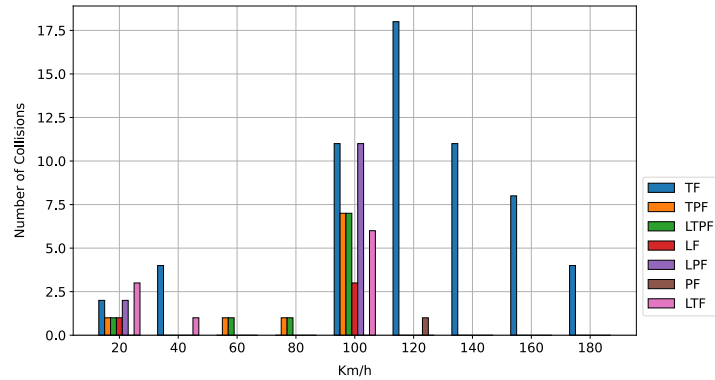
Figure 8. Number of collisions per speed.
