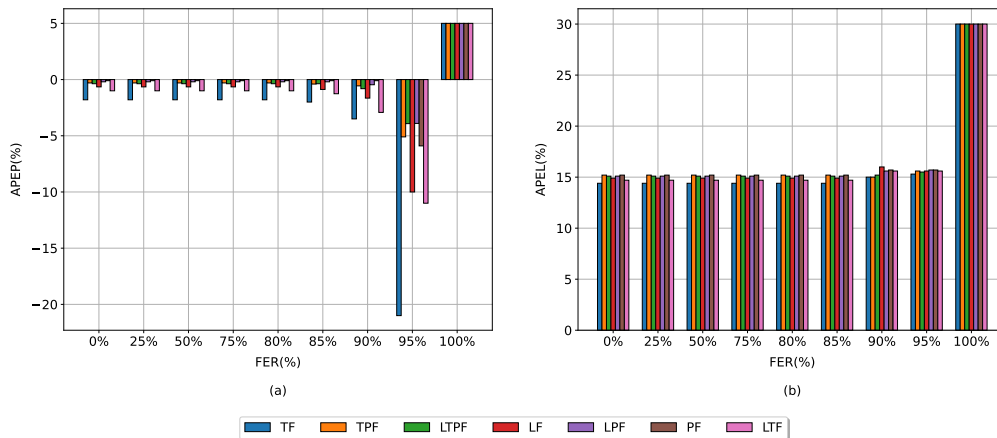
Figure 3. APEP and APEL metrics for a Low Speed scenario.
