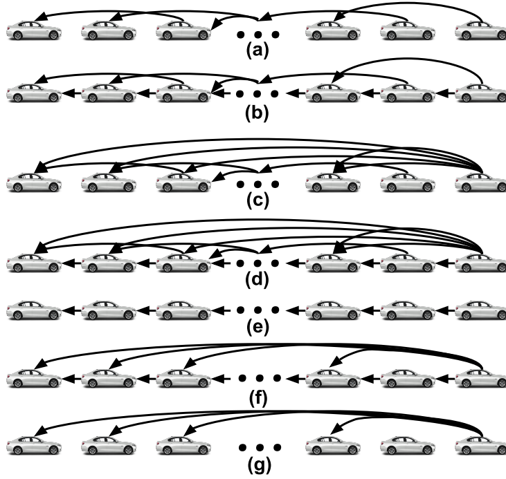
Figure 2. IFTs analyzed: (a) TF, (b) TPF, (c) LTF, (d) LTPF, (e) PF, (f) LPF, and (g) LF.
