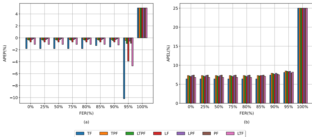
Figure 6. APEP and APEL metrics for an Ultra High Speed scenario.
