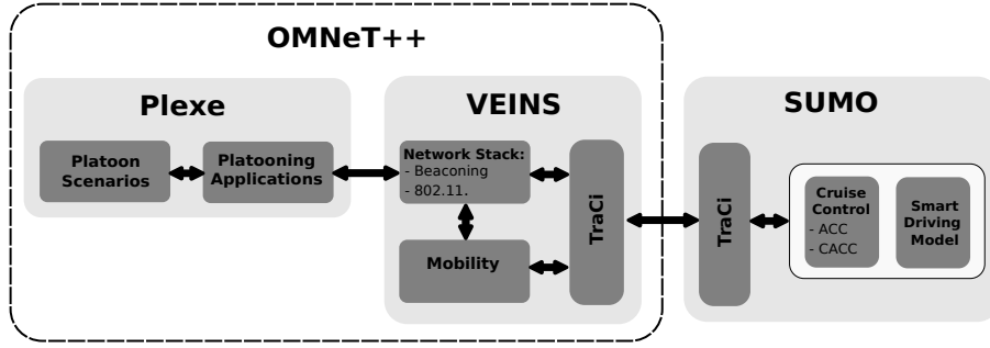
Figure 1. Framework architecture for platoon simulation.
