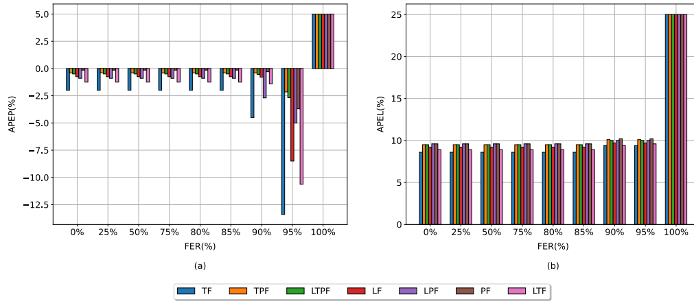
Figure 5. APEP and APEL metrics for a High Speed scenario.
