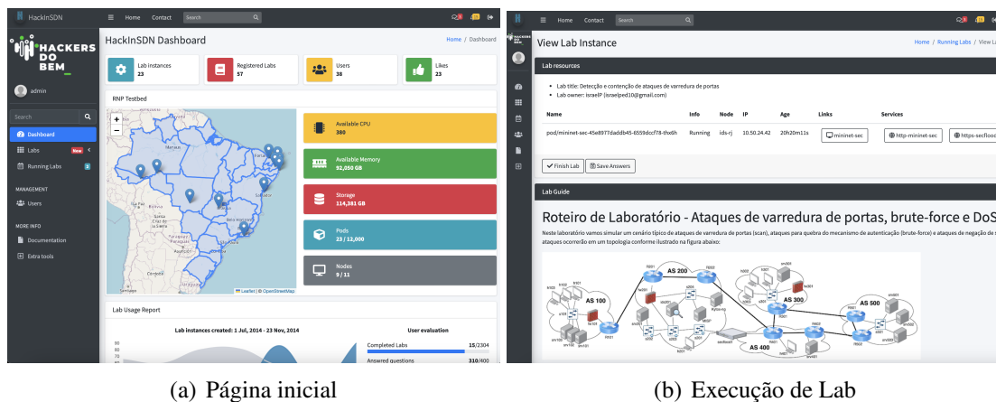
Figura 3. Interface web do Dashboard HackInSDN
