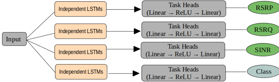
Figure 1. Architecture of the STL model.
