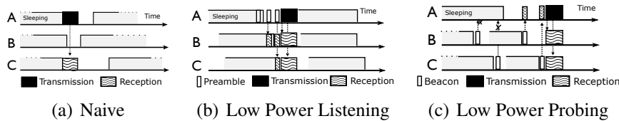
Figure 2. Symbiotic design of duty-cycling and opportunistic routing for UWSNs.
