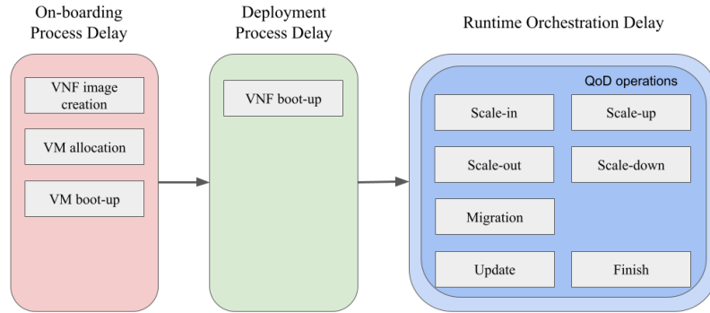
Figura 3. Slicing Operations lifecycle. Adapted from [Yilma et al. 2020]
