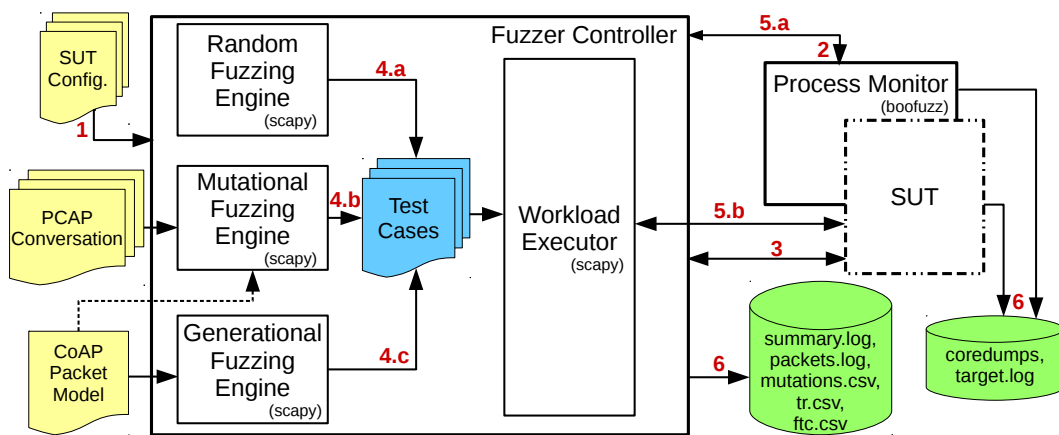
Figure 2. Architecture of the testing system.
