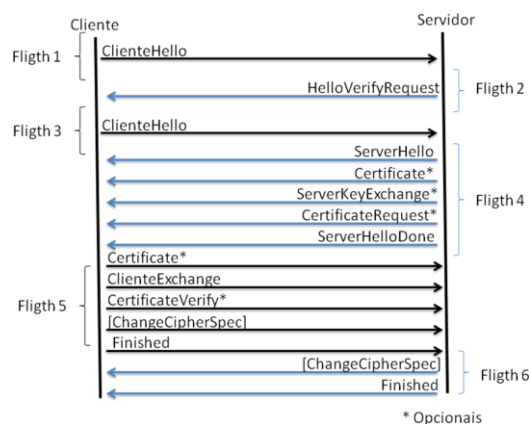
Figura 1 - Flights do Handshake no DTLS
