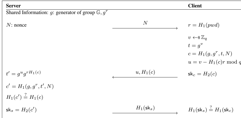
Figure 1. zkPAKE Protocol.
