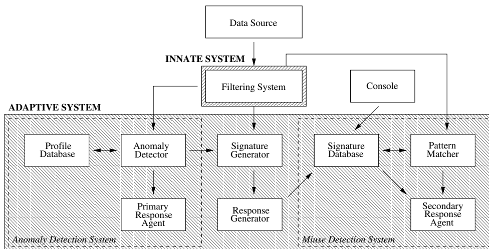
Figure 2: Analogy between innate, adaptive systems and the proposed IDS.
