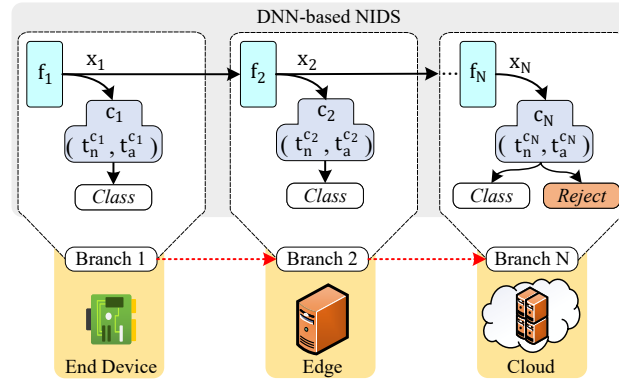
Figure 2: Workflow of the proposed DNN-based NIDS, illustrating early-exit-enabled intrusion detection offloading in EC environments.
