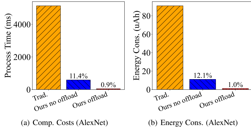
Figure 4: Average per-event inference time and energy consumption at the End Device comparing full on-device DNN execution, proposed early-exit with no offloading, and offloading to the Cloud.
