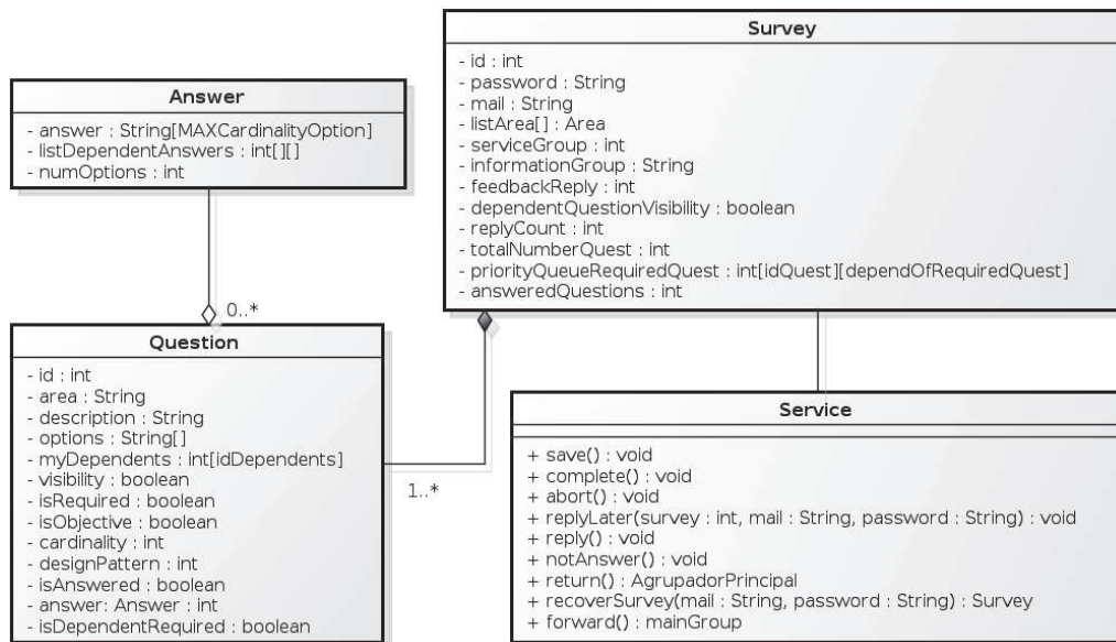
Figura 3. Domain Model for Survey Applications
