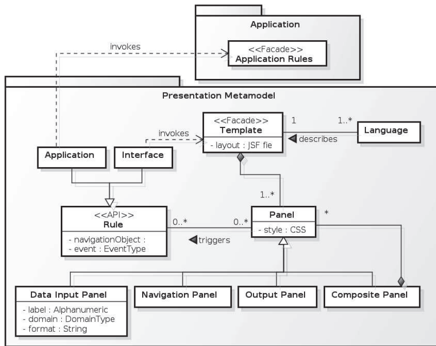
Figura 2. Presentation Metamodel
