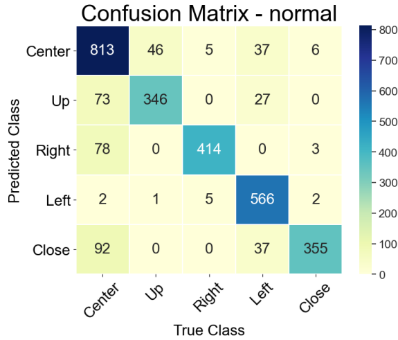
Fig. 8. Confusion matrix for the five directions.
