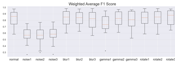
Fig. 9. Weighted average F1 Score of the transformations.
