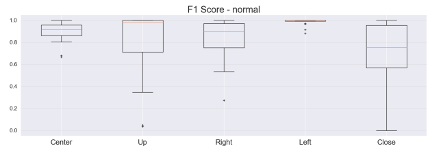
Fig. 7. F1 Score for the 5 directions obtained with original dataset.
