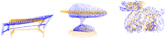
Figure 4: Examples of artificial deformations created by our adopted self-supervised training approach. The original point cloud is in blue while the deformed one is in orange. Notice that by keeping a pointwise correspondence, we can generate Cropped , Holes , and Outliers point clouds.
