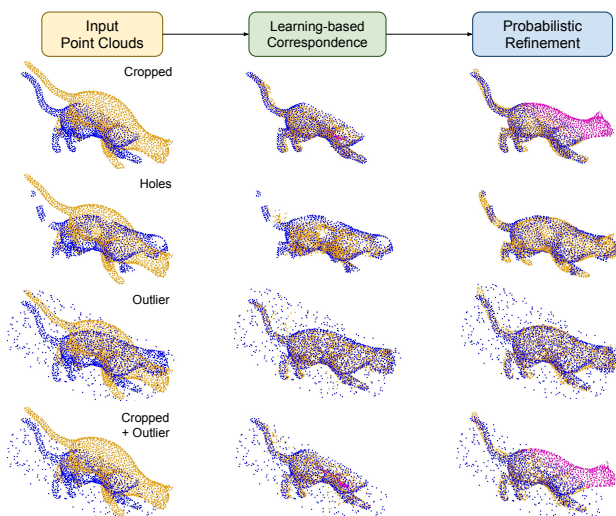
Figure 1: Non-rigid registrations produced by our method for challenging scenarios. We present the results after each stage of our pipeline. The source clouds are in orange and the target ones are in blue. Points without correspondence in the target are shown in magenta.
