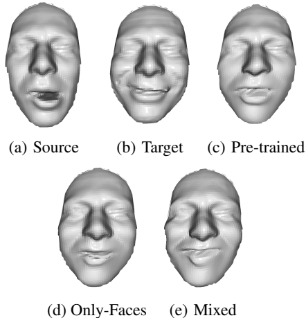
Figure 5: Registering facial expressions using source (a) and target (b) point clouds. Registration results produced by our model trained on: the Custom dataset (c), fine tuning the weights on faces (d), and fine-tuning on faces plus some clouds from Custom (e). The latter keeps the original performance while better dealing with faces.
