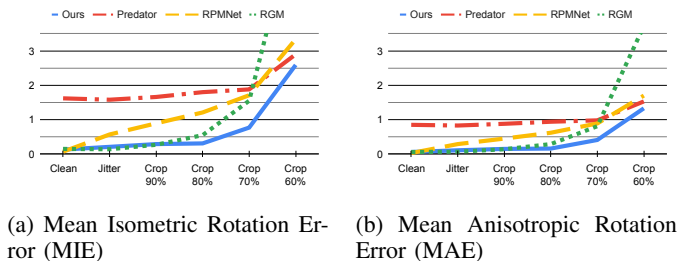
Figure 7: Rotation errors in degrees, MIE and MAE, comparing different approaches for rigid registration on ModelNet40 dataset on Clean , Jitter , and different percentages of samples kept for Crop-Noise .
