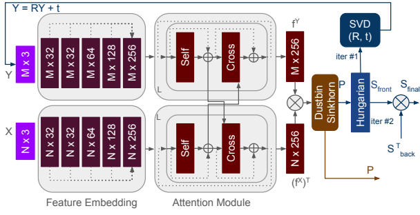
Figure 2: Adapted SuperGlue network for learning-based correspondences. Non-rigid registration uses a single iteration of the purple, red, and brown modules, producing a soft-assignment matrix \mathbf{P} (brown) as output. For rigid registration, the network includes all modules, and it performs two iterations, producing a hard assignment matrix \mathbf{S}_{final} as output.
