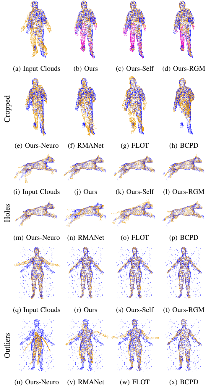
Figure 3: Results on Cropped , Holes , and Outlier types of point clouds on top of the RMANet dataset. Source cloud is in orange and target is in blue. Source points classified as having no matches are shown in magenta.
