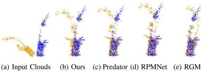
Figure 6: Rigid registration produced by various models.
