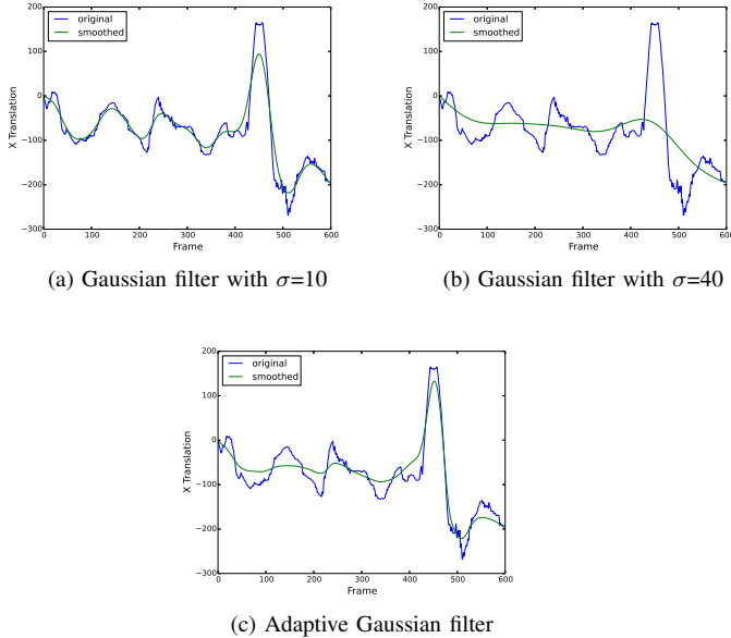
Figure 4. Smoothing of camera motion trajectories.
