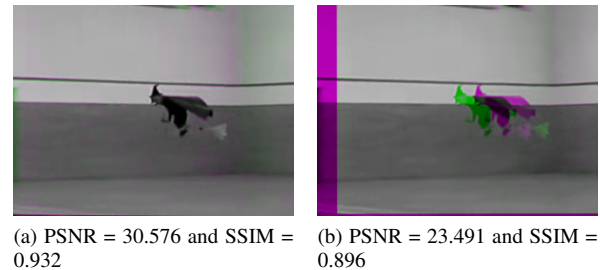
Figure 2. Different matches for the 40th frame of video ours7 .
