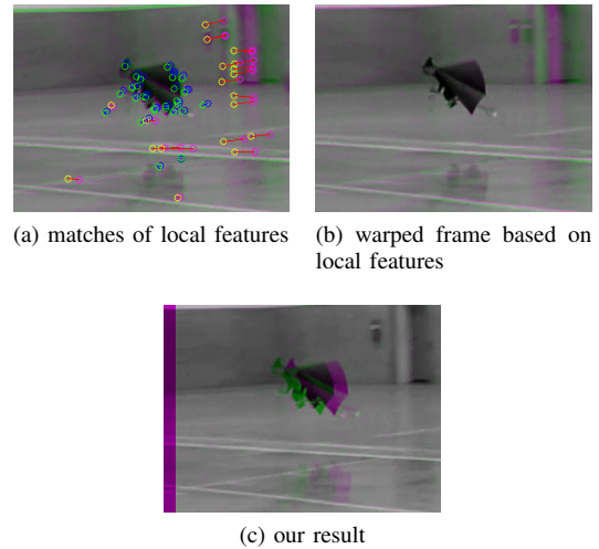
Figure 1. Motion estimation for the 129th frame of video ours6 .
