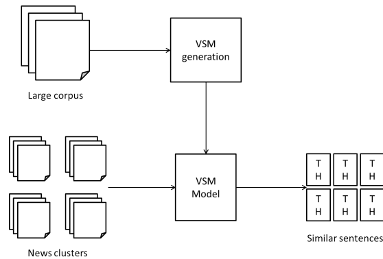
Figure 2. Similar sentence extraction process.
