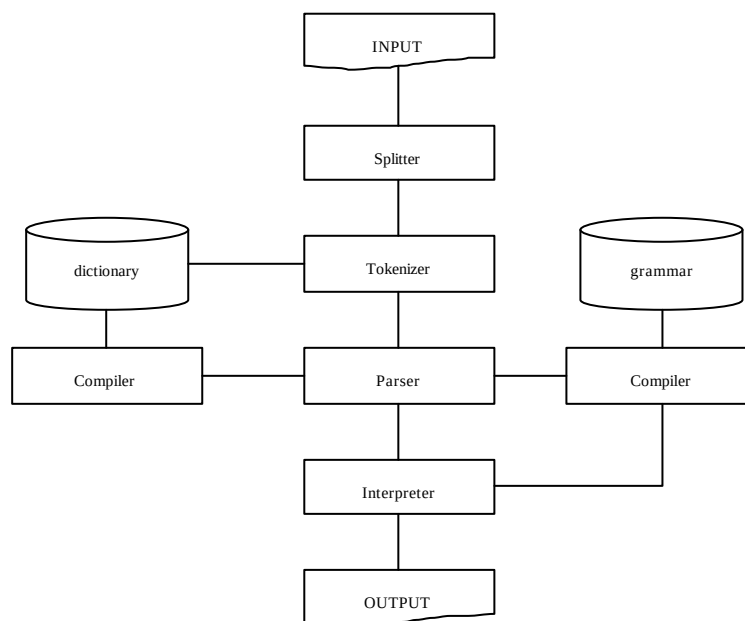
Figure 1. HERMETO's architecture
