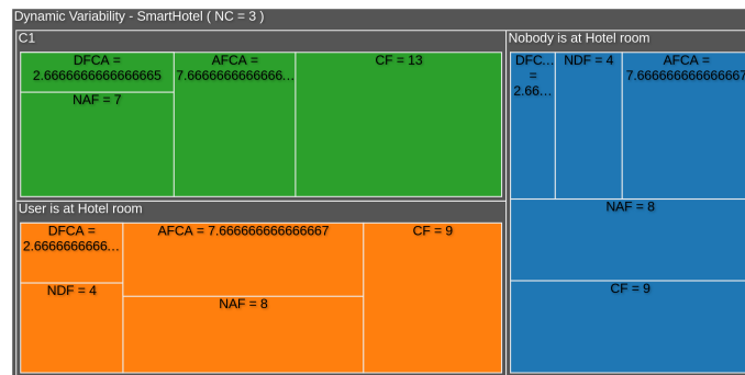
Figure 2. Visualizing the dynamic variability.
