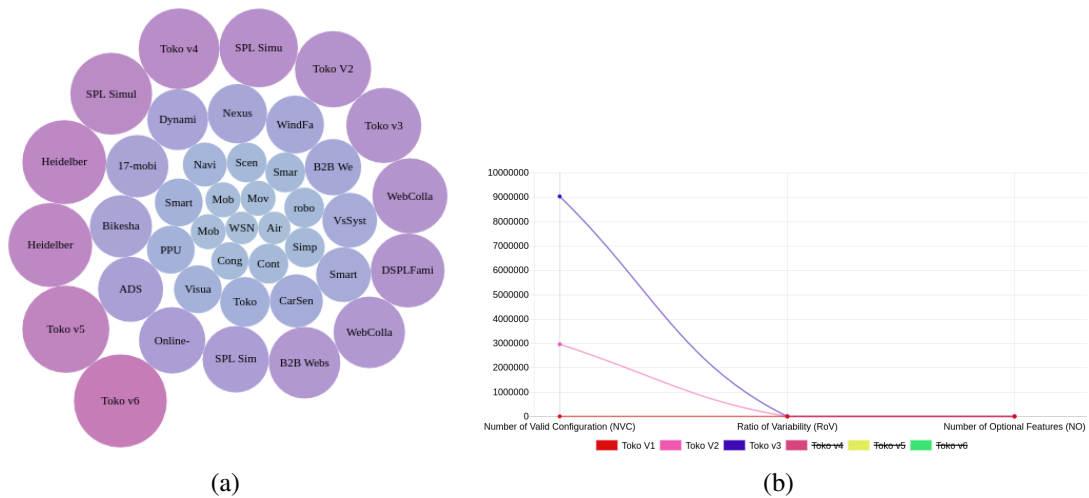
Figure 1. (a) Visualizing the extensibility of FMs e (b) Visualizing the static variability of the FM versions
