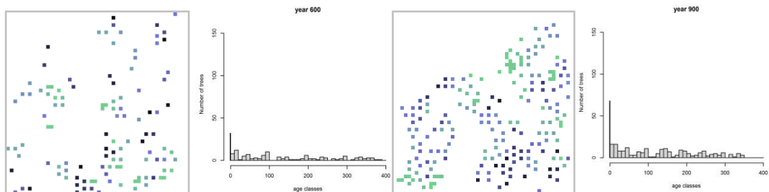
Figure 3. Simulation with fire disturbance: Araucaria population after 600 and 900 years; histograms showing respective age classes.
