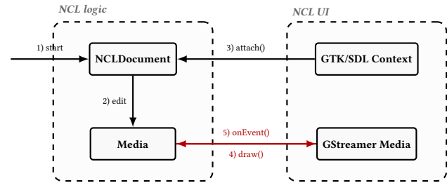
Figure 3: Traditional native C++ NCL player architecture describing PUC-Rio Ginga v0.13 and v1.0, demonstrating tight coupling between logic elements and UI graphics bindings.
