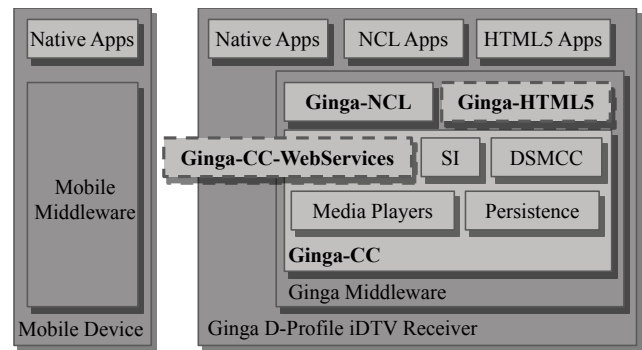
Figure 2: D-Profile Ginga Receiver (Source: [11]).
