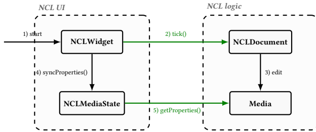
Figure 5: gingaf communication diagram
