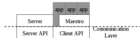
Figure 2: MARS architecture.
