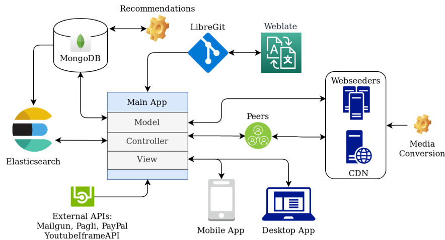
Figure 1: Libreflix architecture
