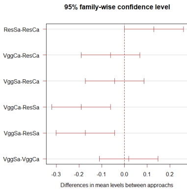
Fig. 4. Graph representing the difference in average performance levels for Recall between approaches.
