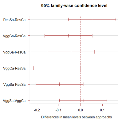
Fig. 8. Graph representing the difference in average performance levels for F-measure between approaches
