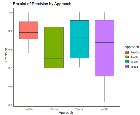
Fig. 3. Boxplot relating approach to Precision metric.
