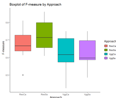
Fig. 9. Boxplot relating the approach to F-measure.
