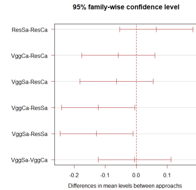
Fig. 6. Graph representing the difference in average performance levels for Accuracy between approaches
