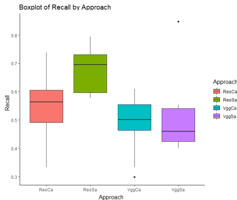
Fig. 5. Boxplot relating the approach to Recall metric.
